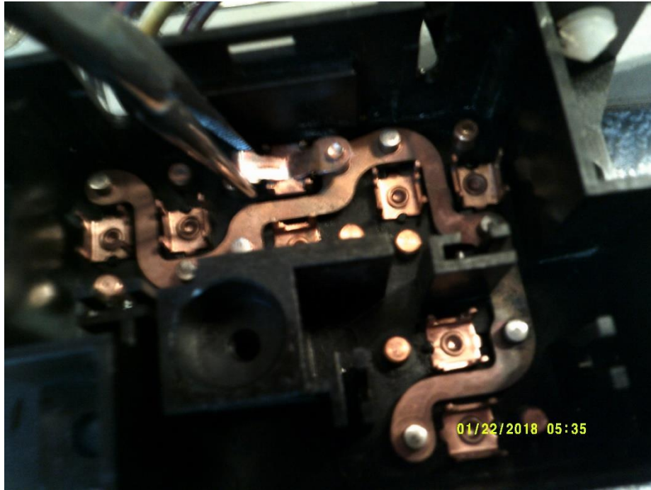
Removing one of the contact pieces.
